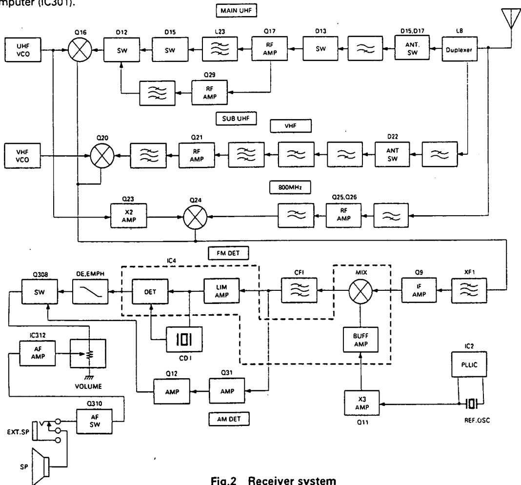
Fig.2 Receiver system
