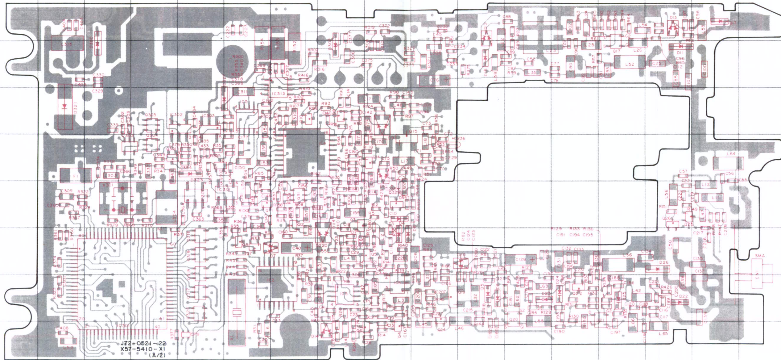
TX-RX UNIT (X57-5410-XX) (A/2)Foil Side View -11:K,K2,-21:T,E,E3,M2,M3,M4
