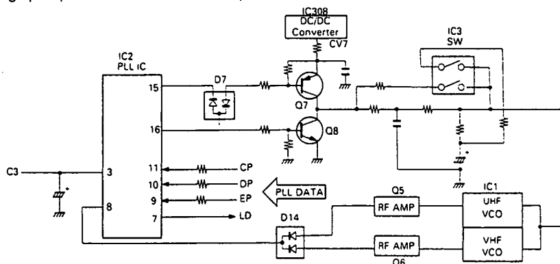
Fig.5 PLL circuit
