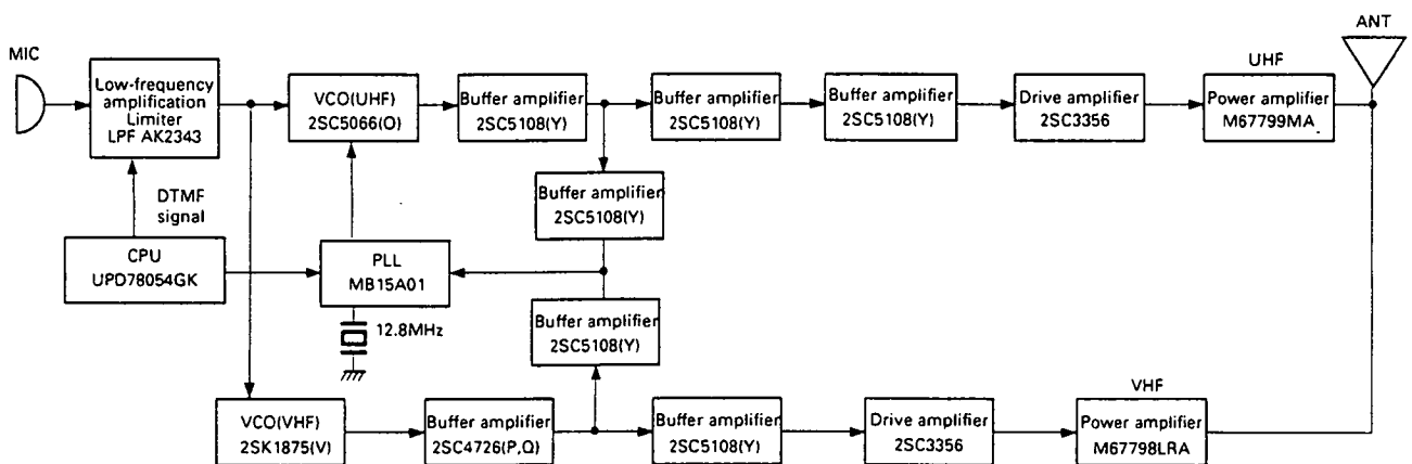
Fig.3 Transmitter system
