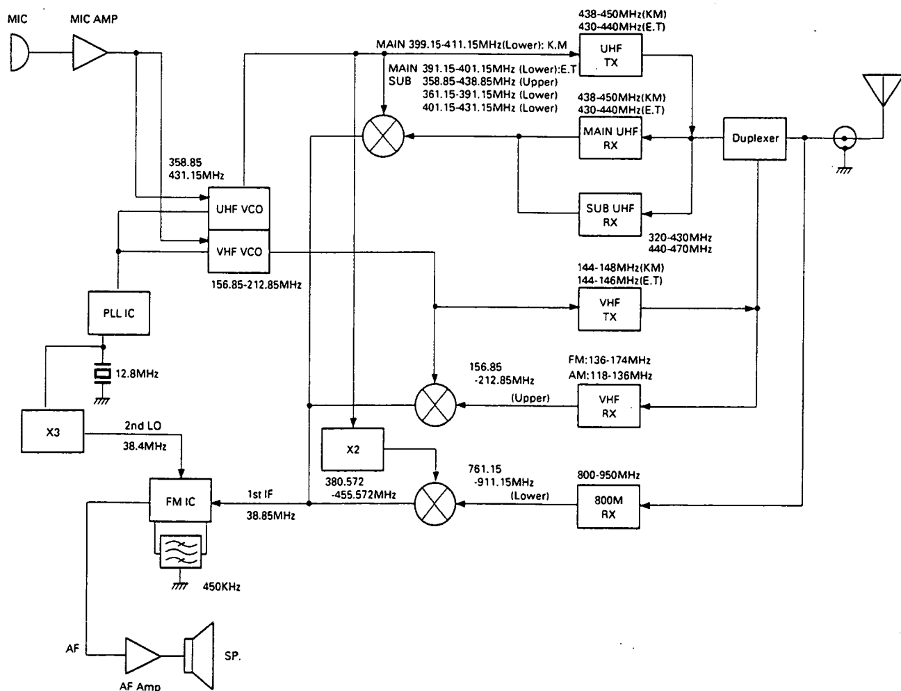
Fig.1 Frequency configuration
